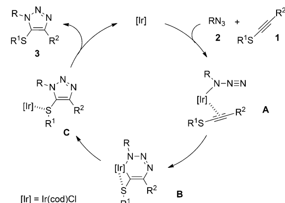
Scheme 2. Proposed mechanism.
